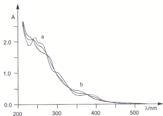
Fig. 5. Spectral changes during the photolysis of 5.04 \times 10^{-5} M \text{Rh}(\text{phpy})_2(\text{axt}) in EtOH at r.t. after 0 (a), 40, and 80 (b) min irradiation time with \lambda_{\text{irr}} = 254 nm, 1 cm cell.
