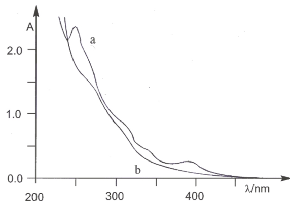
Fig. 6. Spectral changes during the photolysis of 5.25 \times 10^{-5} M \text{Rh}(\text{phpy})_2(\text{axt}) in \text{CH}_2\text{Cl}_2 at r.t. after 0 (a) and 180 (b) min irradiation time with \lambda_{\text{irr}} = 254 nm, 1 cm cell.
